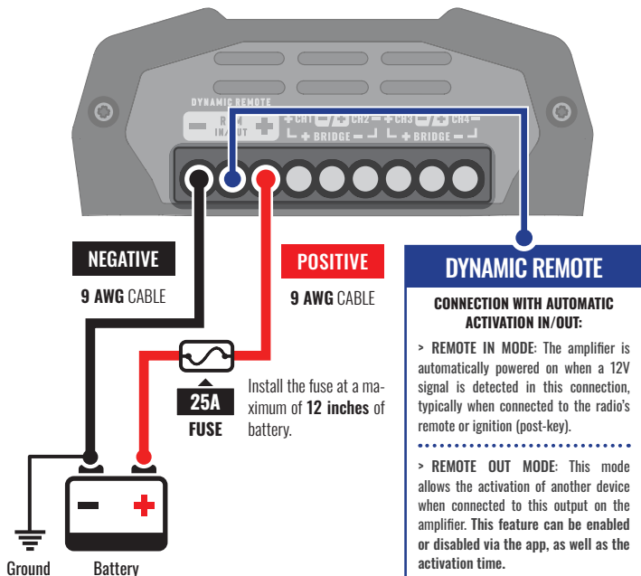
SIDEVIEW (POWER)
